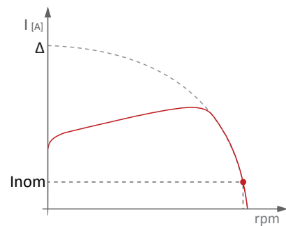
Current trend with accessory Electronic soft-starter
