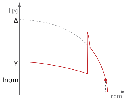
Current trend without accessory Electronic soft-starter
