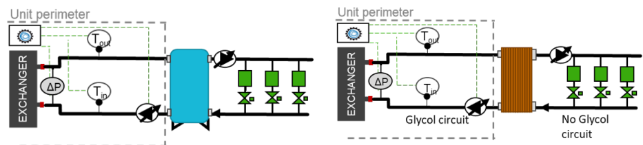
FLOWZER VPS with DT-based control
