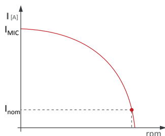
Current trend without accessory
