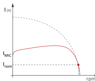
Current trend with accessory Electronic soft-starter
